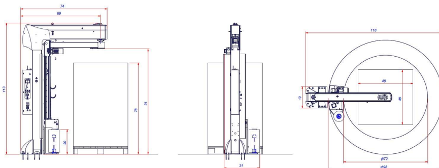
LAYOUT MASTERWRAP HD [inch]
